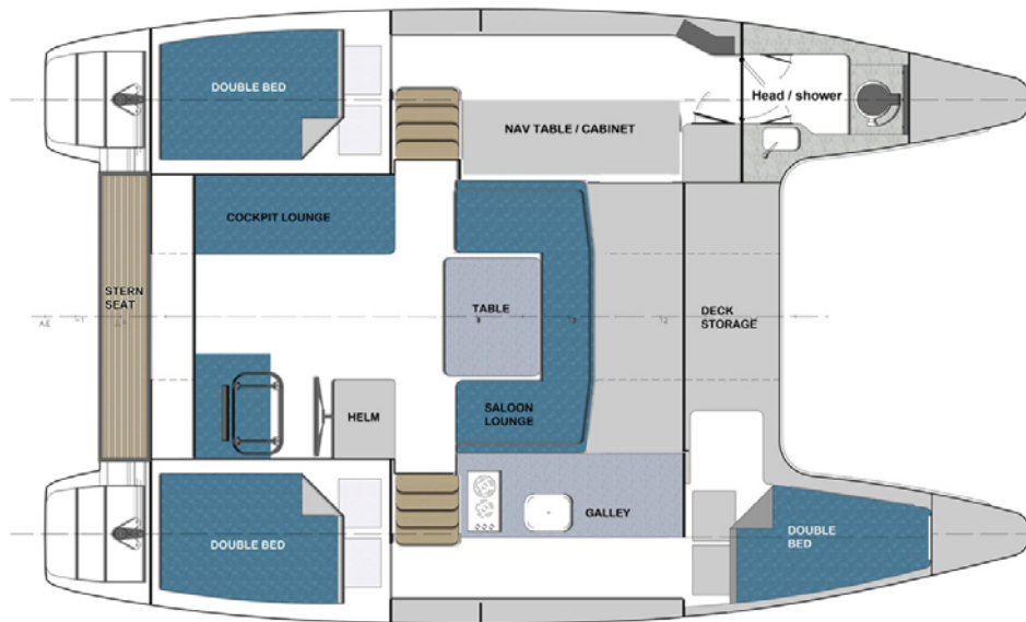
3 cabin & 1head
