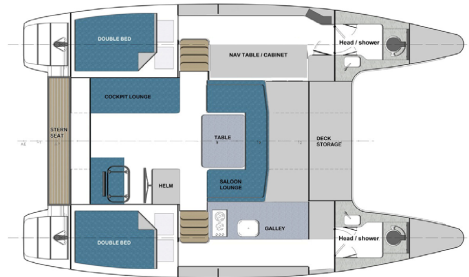
2 cabin & 2 head
